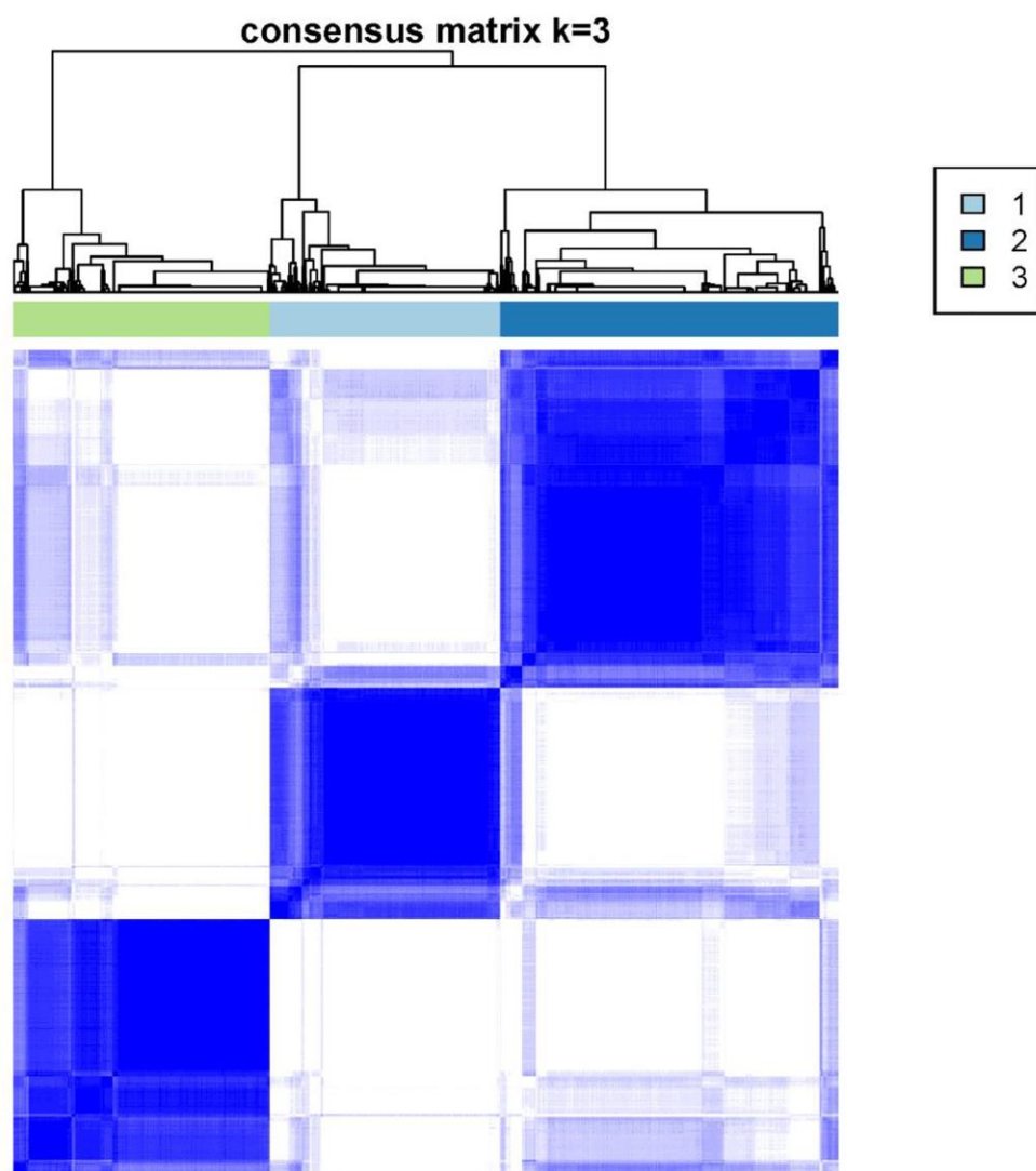
Supplementary Figure 2. Heatmap showing the consensus matrix for a clustering solution with k = 3 clusters.
