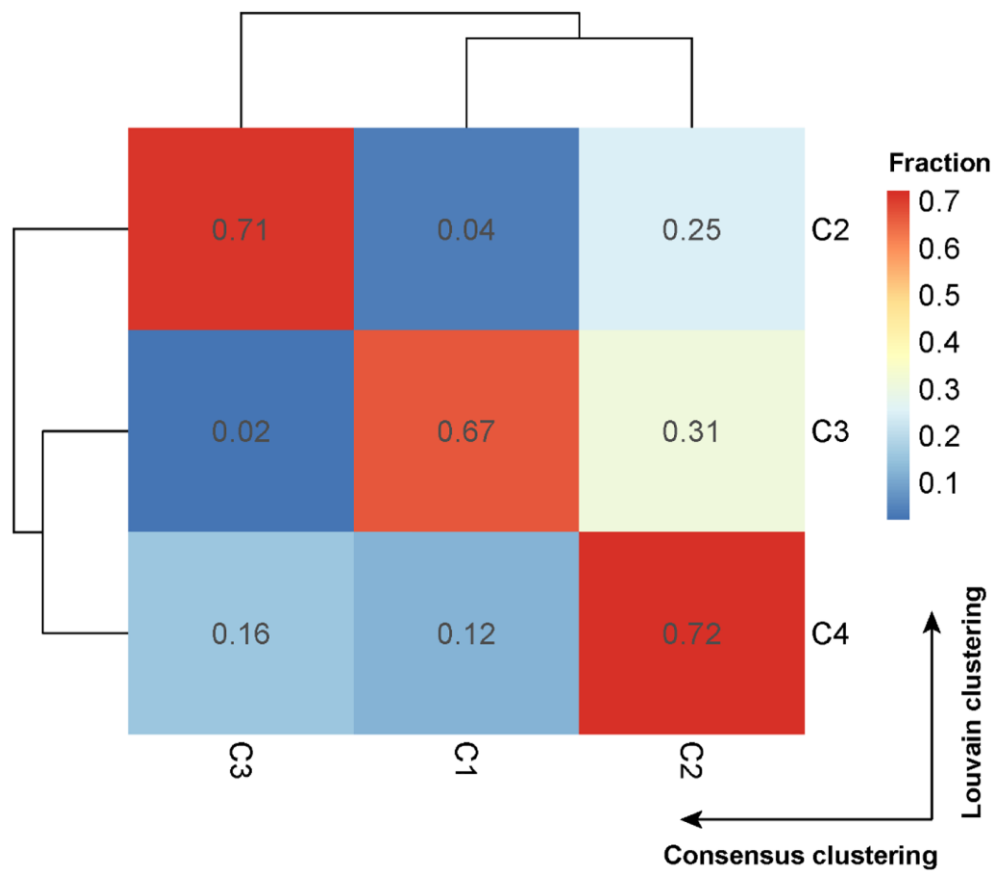
Supplementary Figure 3. Heatmap showing the degree of consistency between the clusters identified by the Louvain algorithm and those identified by consensus clustering. Each cell in the heatmap represents the agreement level for a pair of items regarding their cluster assignments across both methods.
