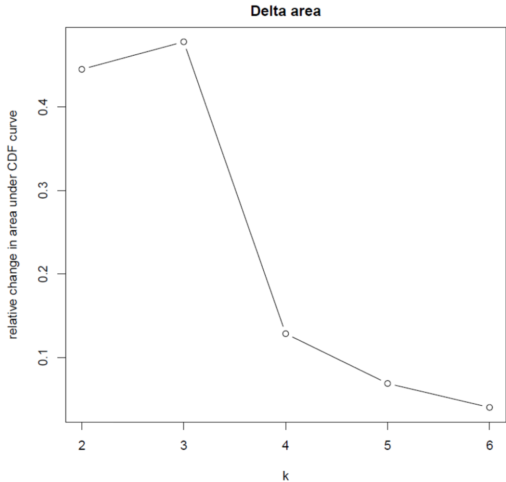
Supplementary Figure 1. Delta area plot showing the relative change in area under the cumulative distribution function (CDF) curve for different numbers of clusters ( k ) in a consensus clustering analysis.
