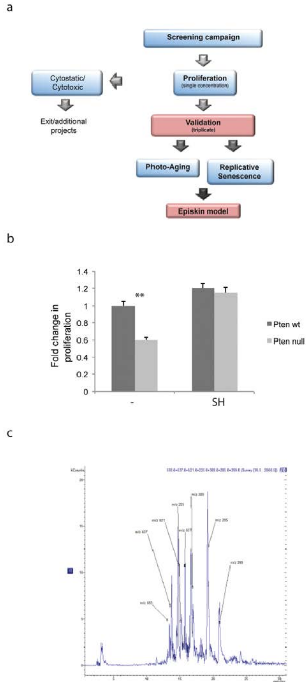
Supplementary Figure S1. (a) Schematic representation of PICCS assay First step is the identification of candidate compounds that have an anti-senescent effect in the in vitro PICCS assay (screening campaign). Compounds are tested for their effect on proliferation and b-gal expression in primary murine embryonal fibroblasts (MEFs) lacking Pten gene ( Pten null). The candidate compounds that are able to increase growth rate more than 40% compared to control and at the same time block senescence (determined by less b-gal positive cells), are selected for testing their ability to block photo-induced and replicative senescence in human fibroblasts (validation). Cytotoxic compounds instead, are selected for external projects on anti-tumor therapy. Candidate compounds that demonstrate efficiency in prevention of replicative and photo ageing are tested in reconstituted skin model as part of preclinical development. Successful (non toxic and non irritant) candidates are formulated into topical products and proceed to clinical trials. (b) Proliferation of Pten null MEFs in culture after 5 days of treatment with S. haenkei extract. Pten null MEFs were plated in concentration of 2 \times 10^4 cells/ml and treated for 5 days with 10 \mu\text{M} Nutlin-3 or 10 \mu\text{g/ml} SH extract. After this period, the proliferation was determined using Crystal violet staining. (c) An exemplificative chromatogram is reported with the indication of twelve compounds identified on the basis of MSn fragmentations.
