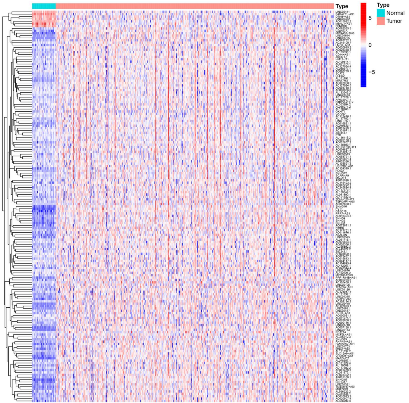
Supplementary Figure 1. Differentially expressed lncRNAs in COAD visualized by a heatmap.
